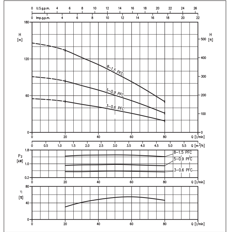
PERFORMANCE CURVES 3TP 3 series impeller diameter: 46 mm (according to ISO 9906 Attachment A)
